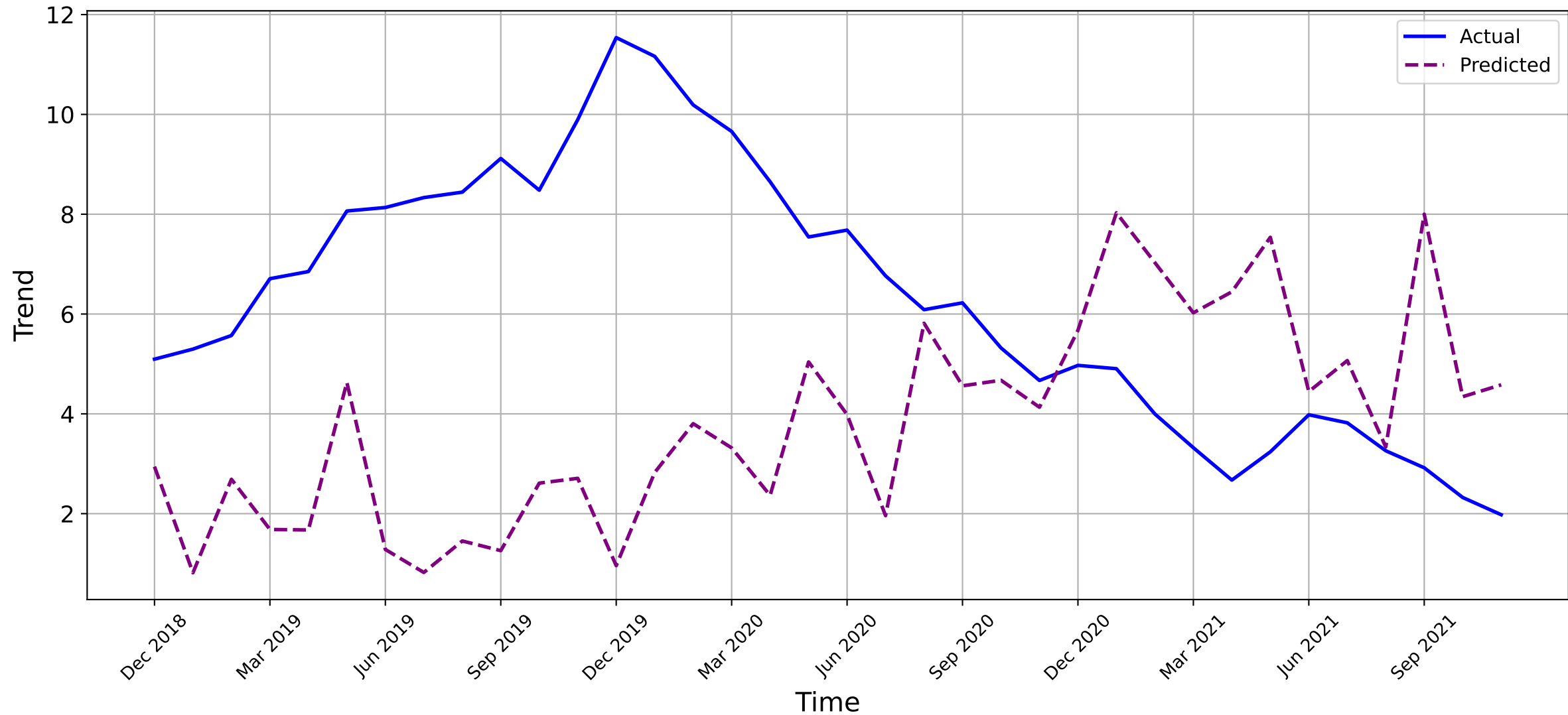
Solution_VULNERABILITY_SCANNER_Mentions - Validation
